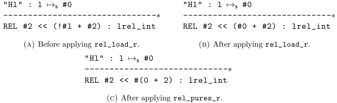
FIGURE 17. Interactive refinement proof of lemma example_load in ReLoC.
