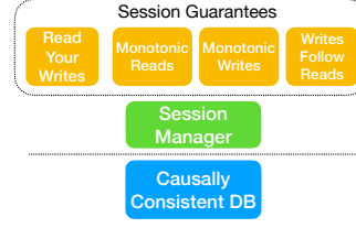
Fig. 10. Vertical compositionality of specifications.
