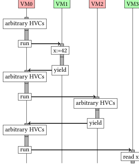
Fig. 8. A compromised primary VM is also contained: memory integrity (illustrating defensive code). This assumes VM1 and VM3 initially exclusively share a page p containing location x .
